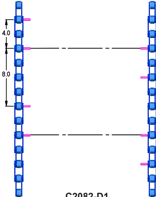
C2082-D1 EXTENDED PIN ORIENTATION
