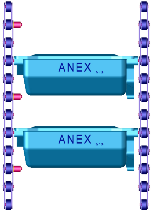
BUCKET INSTALLATION
