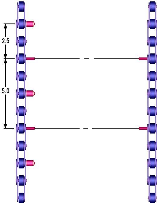
EXTENDED PIN ORIENTATION
